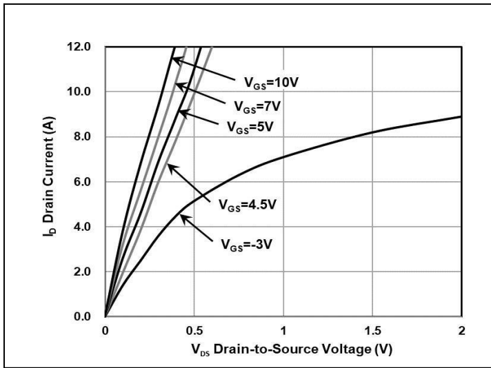
FIG.1-Typical Output Characteristics
