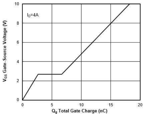
FIG.7-Gate Charge Characteristics
