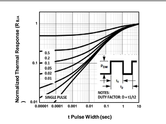
FIG.6-Transient Thermal Impedance
