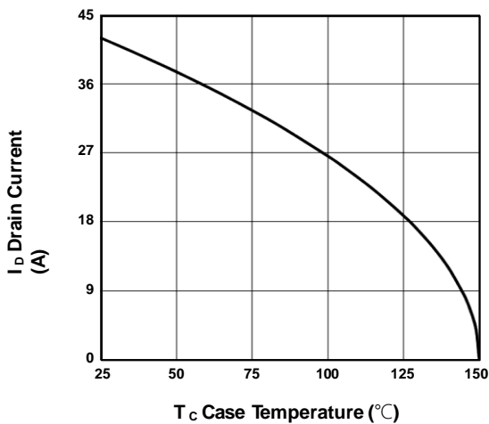
FIG.5-Drain Current vs. T C
