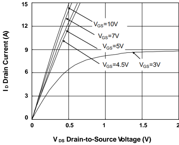
FIG.1-Typical Output Characteristics
