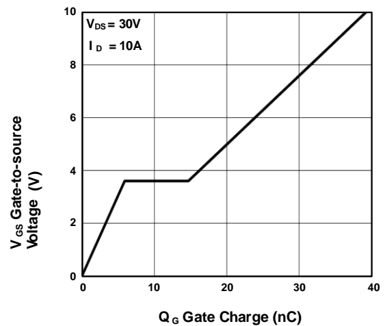
FIG.6-Gate Charge Characteristics
