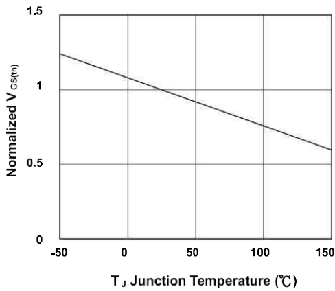
FIG.3-Normalized V_{GS(th)} vs. T_J
