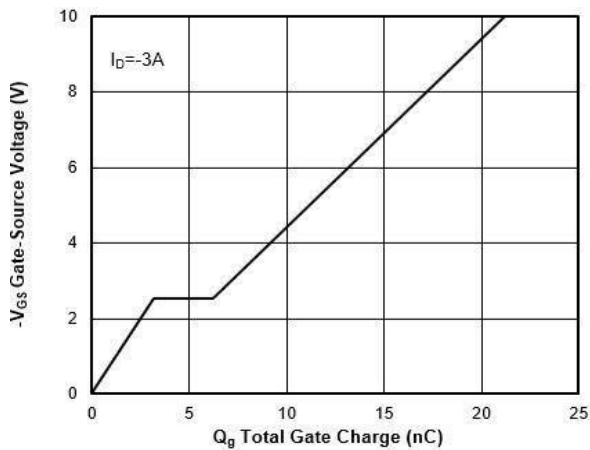
FIG.7-Gate Charge Characteristics
