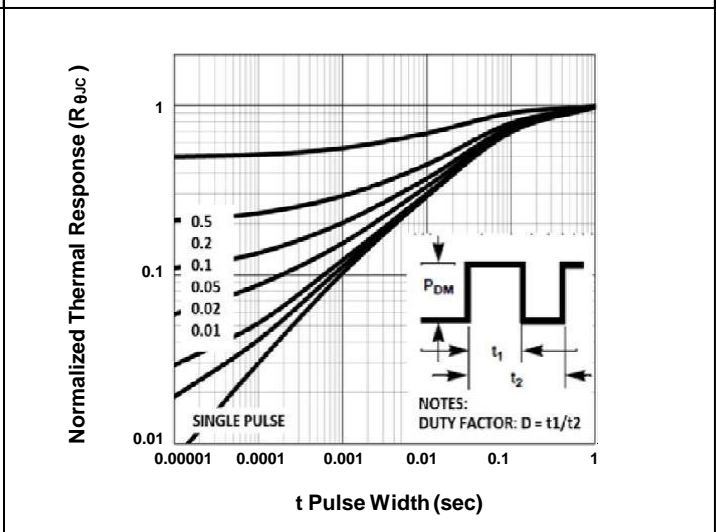
FIG.6-Transient Thermal Impedance
