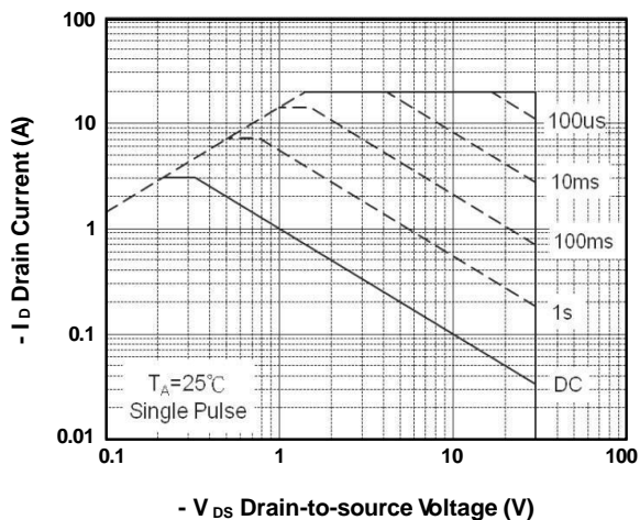
FIG.5-Safe Operating Area
