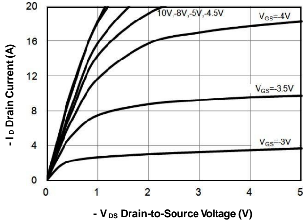
FIG.1-Typical Output Characteristics
