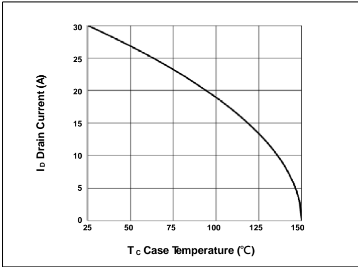
FIG.1-Drain Current vs. T_c
