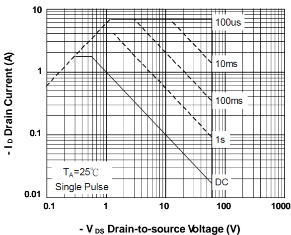
FIG.5-Safe Operating Area
