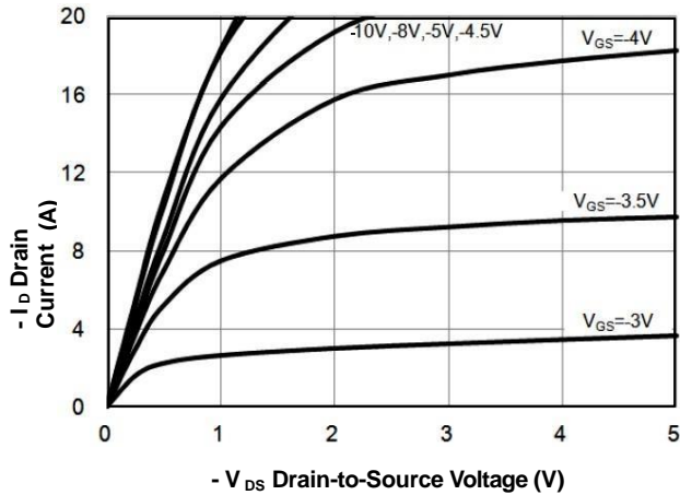
FIG.1-Typical Output Characteristics
