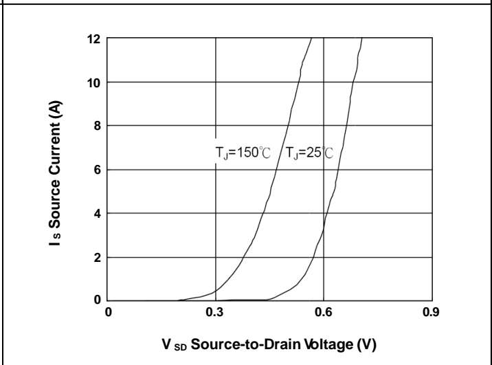
FIG.6-Forward Characteristics of Reverse
