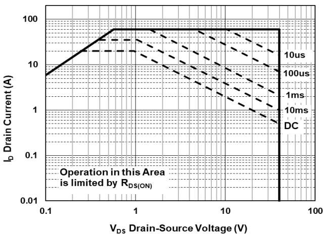
FIG.5-Safe Operating Area
