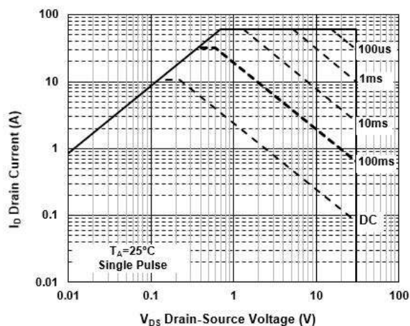
FIG.5-Safe Operating Area
