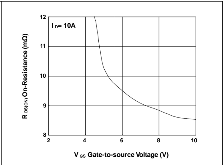
FIG.2-On-Resistance vs. G-S Voltage
