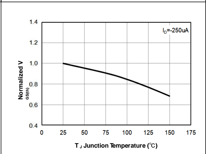
FIG.10-Normalized V_{GS(th)} vs. T_J
