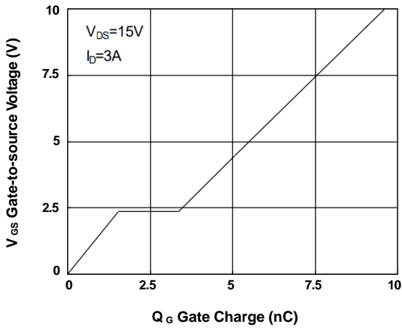
FIG.7-Gate Charge Characteristics
