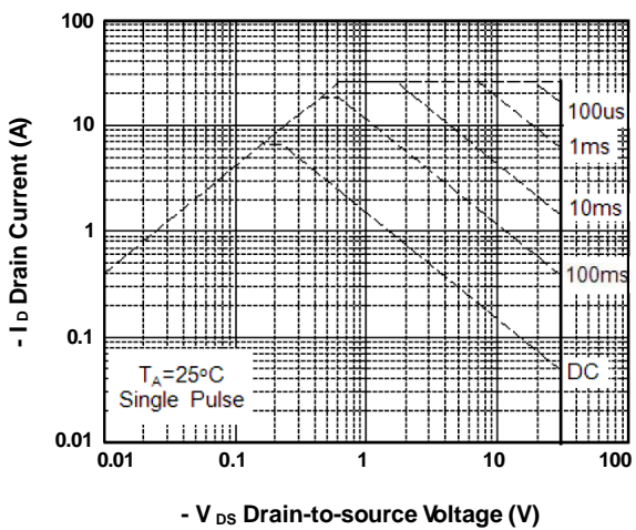
FIG.5-Safe Operating Area
