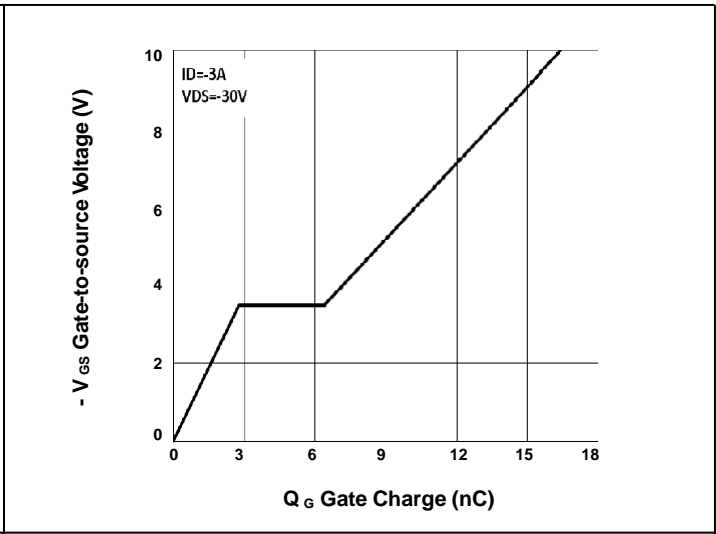
FIG.2-Gate Charge Characteristics
