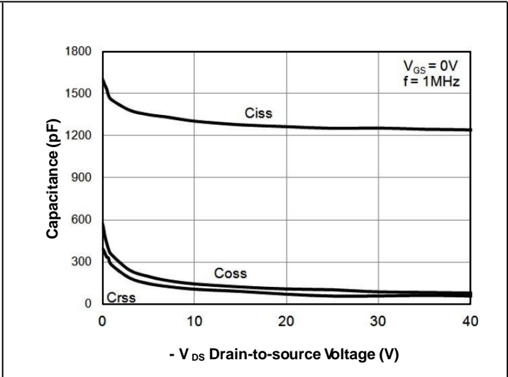
FIG.8-Capacitance Characteristics
