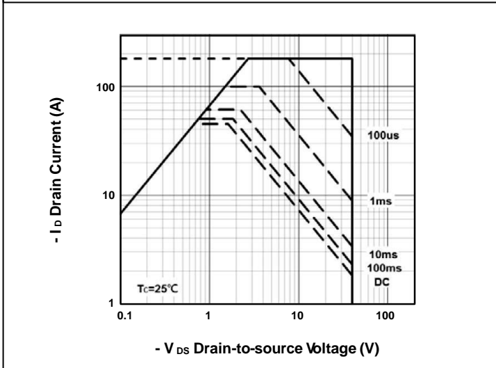
FIG.5-Safe Operating Area
