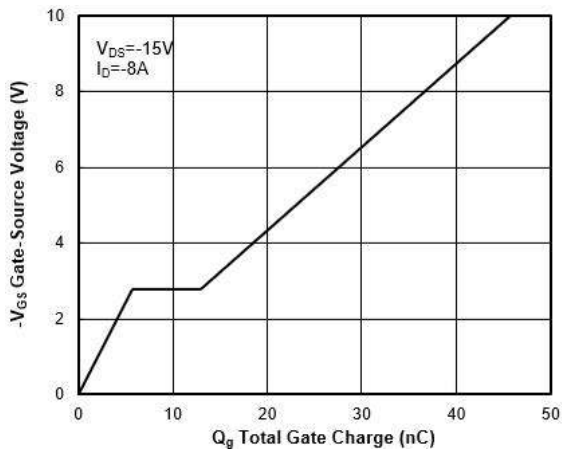
FIG.7-Gate Charge Characteristics
