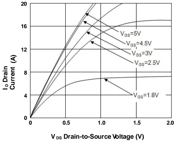
FIG.1-Typical Output Characteristics
