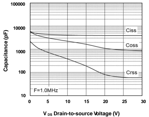
FIG.8-Capacitance Characteristics
