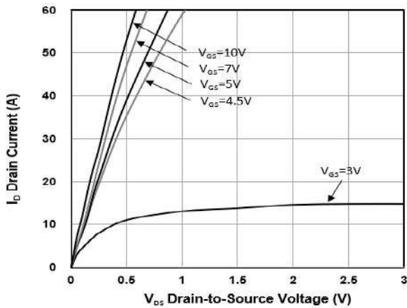
FIG.1-Typical Output Characteristics
