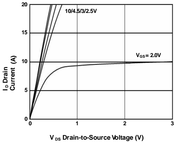
FIG.1-Typical Output Characteristics
