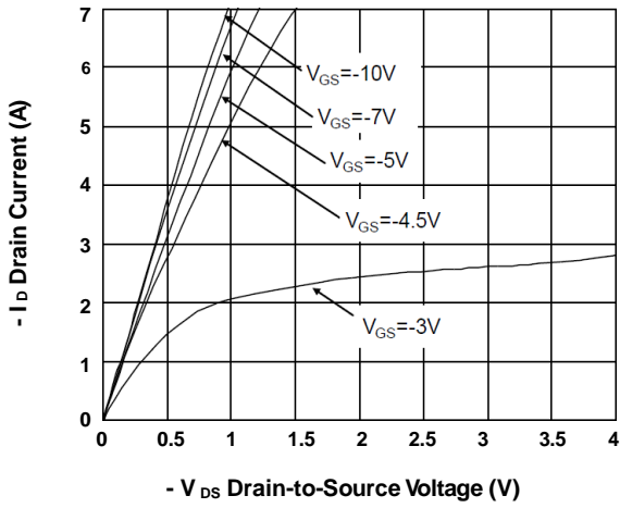
FIG.1-Typical Output Characteristics
