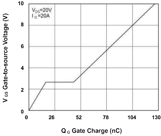
FIG.7-Gate Charge Characteristics
