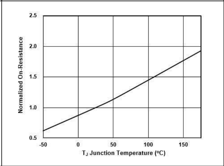
FIG.4-Normalized R_{DS(on)} vs. T_J
