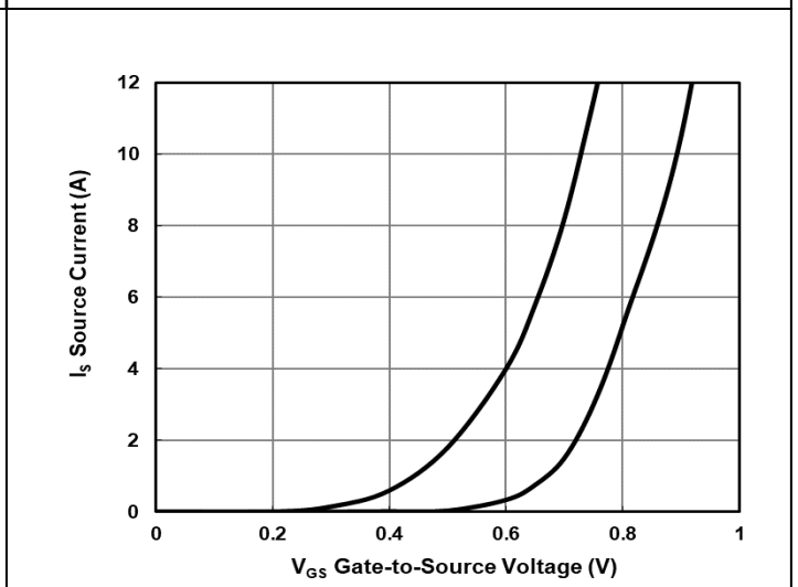
FIG.6-Source Drain Forward Characteristics
