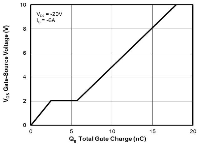
FIG.7-Gate Charge Characteristics
