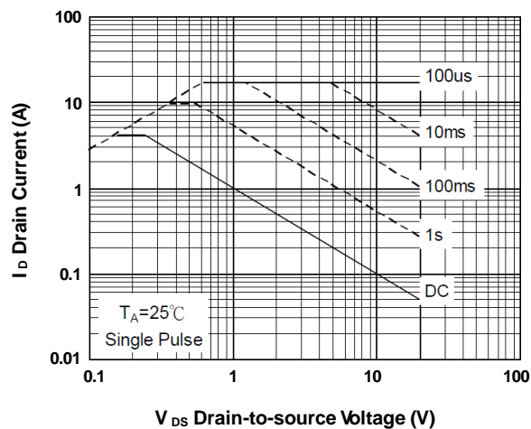
FIG.5-Safe Operating Area
