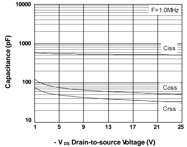
FIG.8-Capacitance Characteristics
