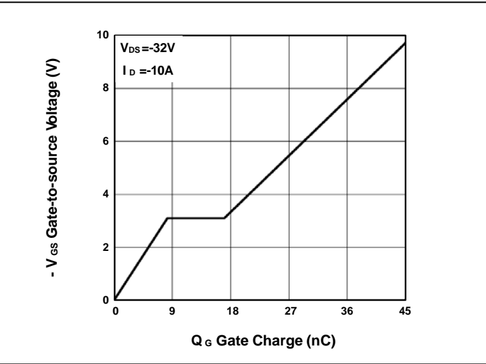
FIG.2-Gate Charge Characteristics
