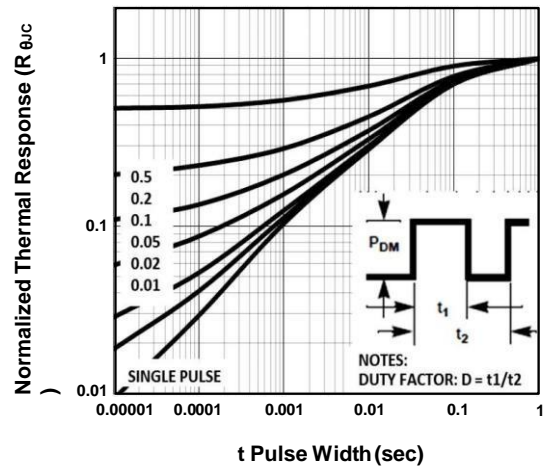
FIG.8-Transient Thermal Impedance
