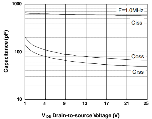
FIG.8-Capacitance Characteristics
