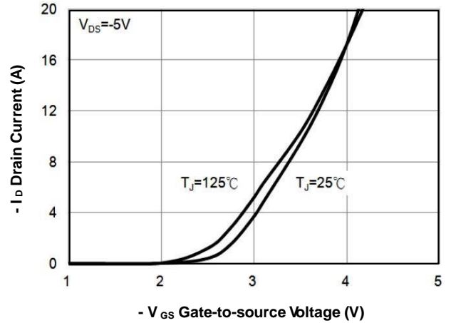
FIG.2-Transfer Characteristics
