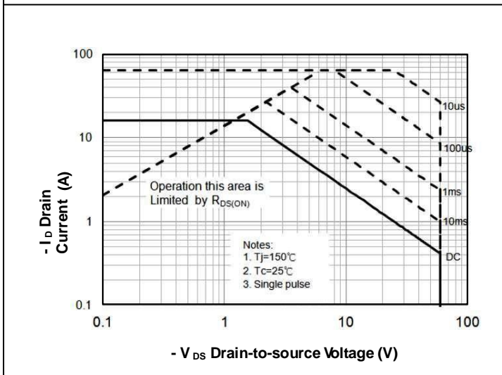
FIG.9-Safe Operating Area
