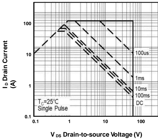
FIG.7-Safe Operating Area
