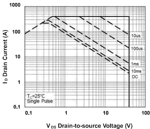
FIG.5-Safe Operating Area
