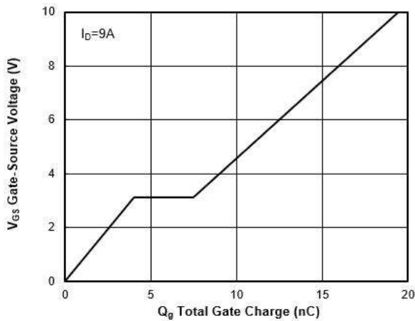
FIG.7-Gate Charge Characteristics
