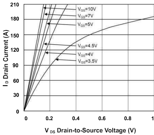
FIG.1-Typical Output Characteristics
