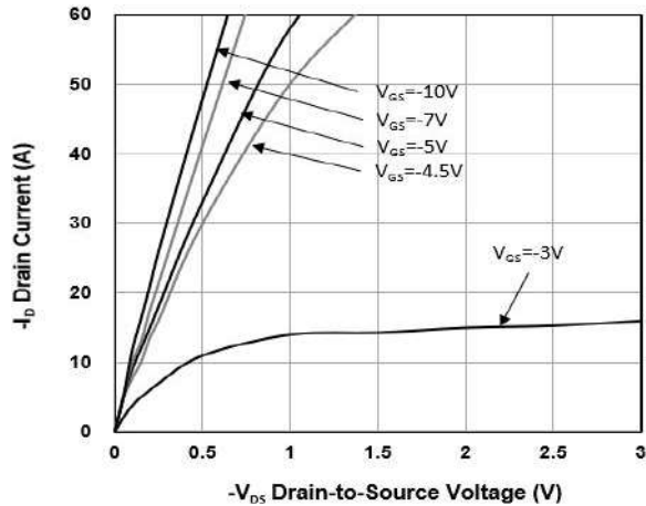
FIG.1-Typical Output Characteristics
