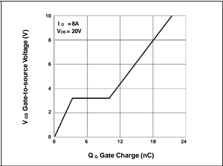
FIG.2-Gate Charge Characteristics
