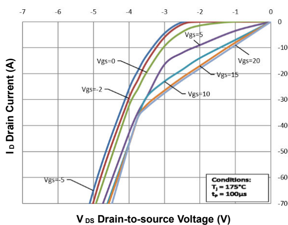
FIG.11- Body Diode Characteristics at T_J = 175^{\circ}C
