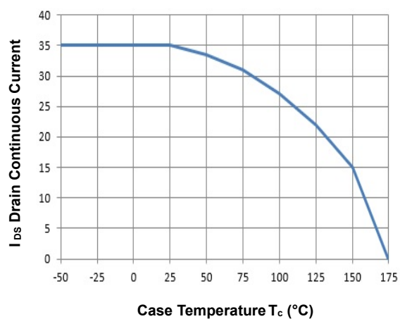
FIG.12- Continuous Drain Current Derating vs. T_c
