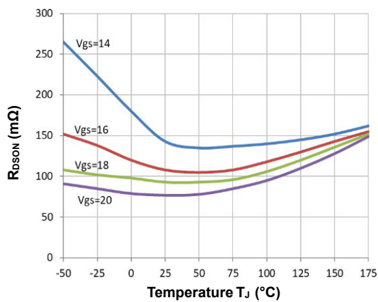
FIG.7- On-Resistance vs. Temperature For Various Gate Voltages
