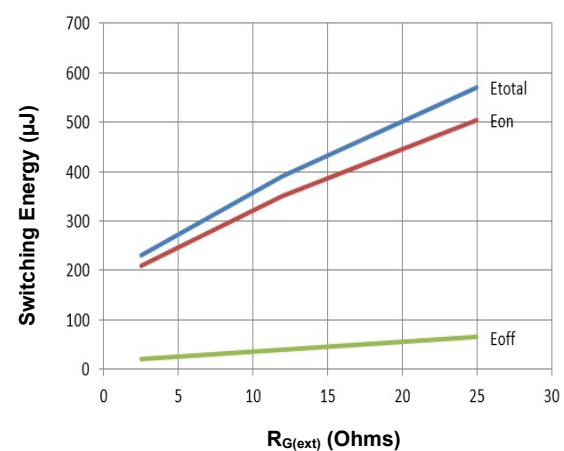
FIG.18- Clamped Inductive Switching Energy vs. R_{G(ext)}
