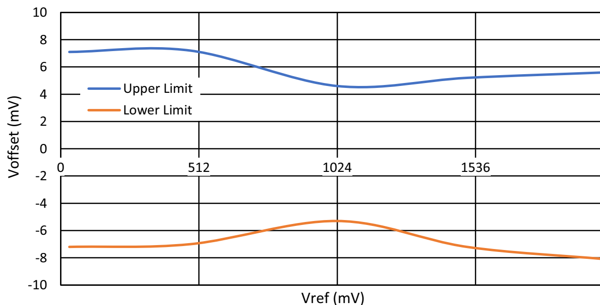
Figure 112: ACMPxH Input Offset Voltage vs. Vref at V_{DD} = 2.3 \text{ V to } 5.5 \text{ V} , T = -40^\circ\text{C to } 85^\circ\text{C} ,
