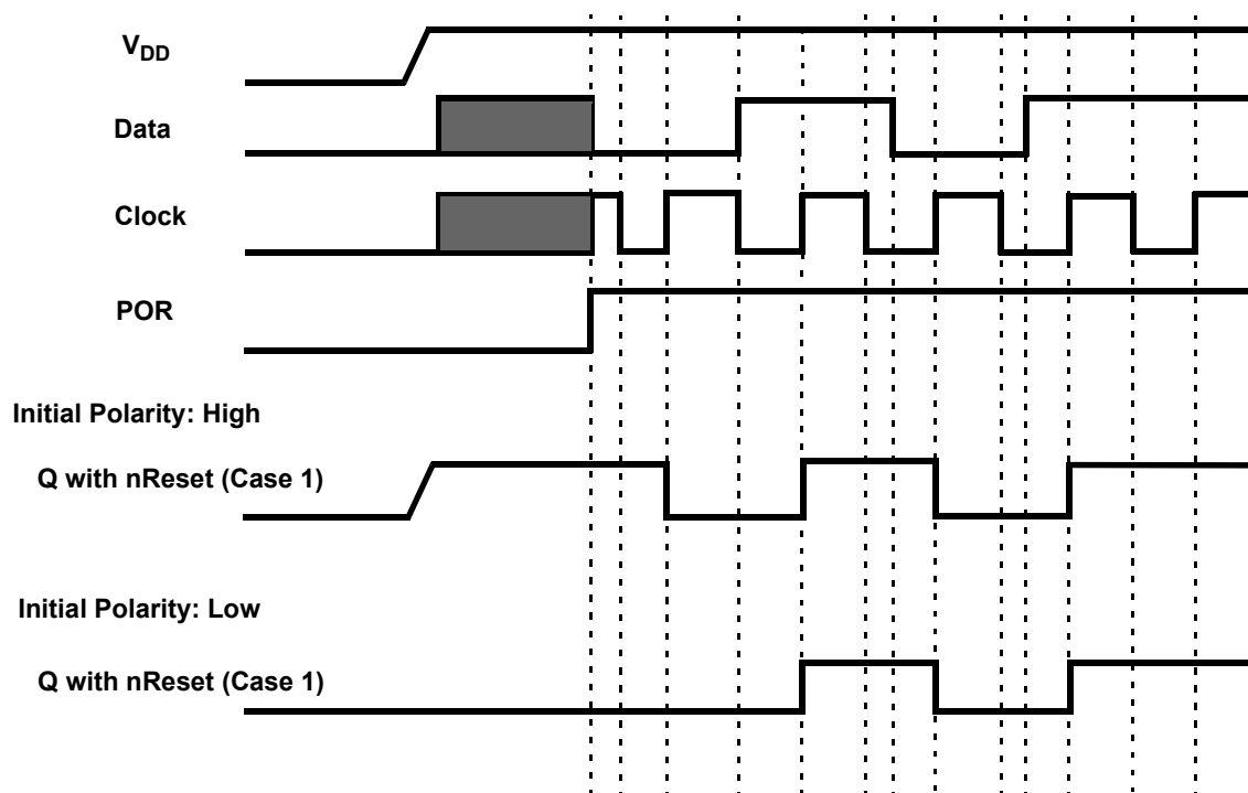
Figure 51: DFF Polarity Operations
