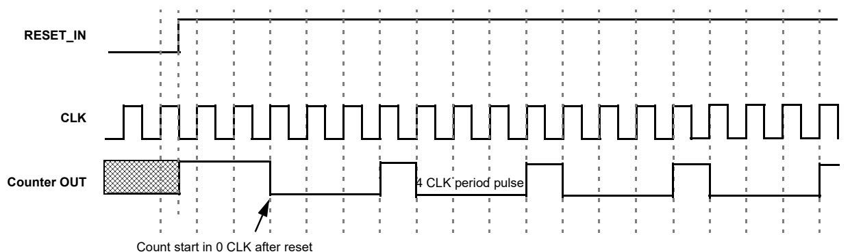
Figure 83: Counter Mode Timing Diagram with Two DFFs Synced Up
