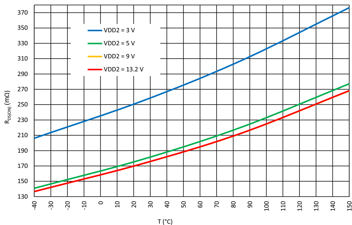
Figure 21: Full Bridge Typical Drain-Source High Side On-Resistance vs. Temperature at I_{LOAD} = 0.5\text{ A} , V_{DD} = 2.3\text{ V}
