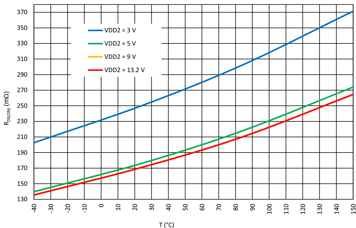
Figure 22: Full Bridge Typical Drain-Source High Side On-Resistance vs. Temperature at I_{LOAD} = 0.5\text{ A} , V_{DD} = 5.5\text{ V}
