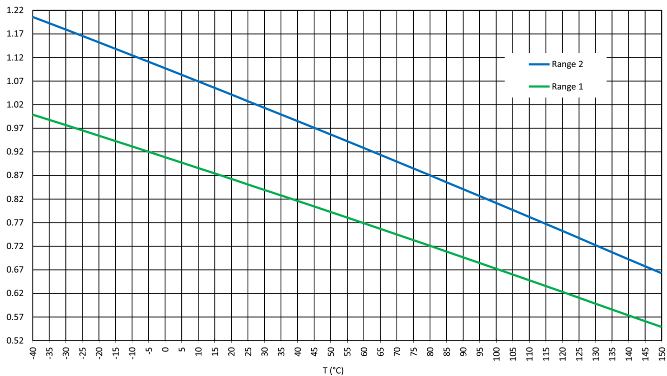
Figure 158: TS Output vs. Temperature, V_{DD} = 2.3 V to 5.5 V
