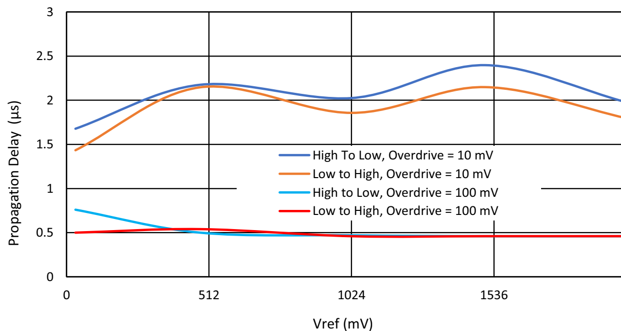
Figure 113: Propagation Delay vs. Vref for ACMPxH at T = 25^\circ\text{C} , at V_{DD} = 2.3 \text{ V to } 5.5 \text{ V} , Gain = 1, Hysteresis = 0
