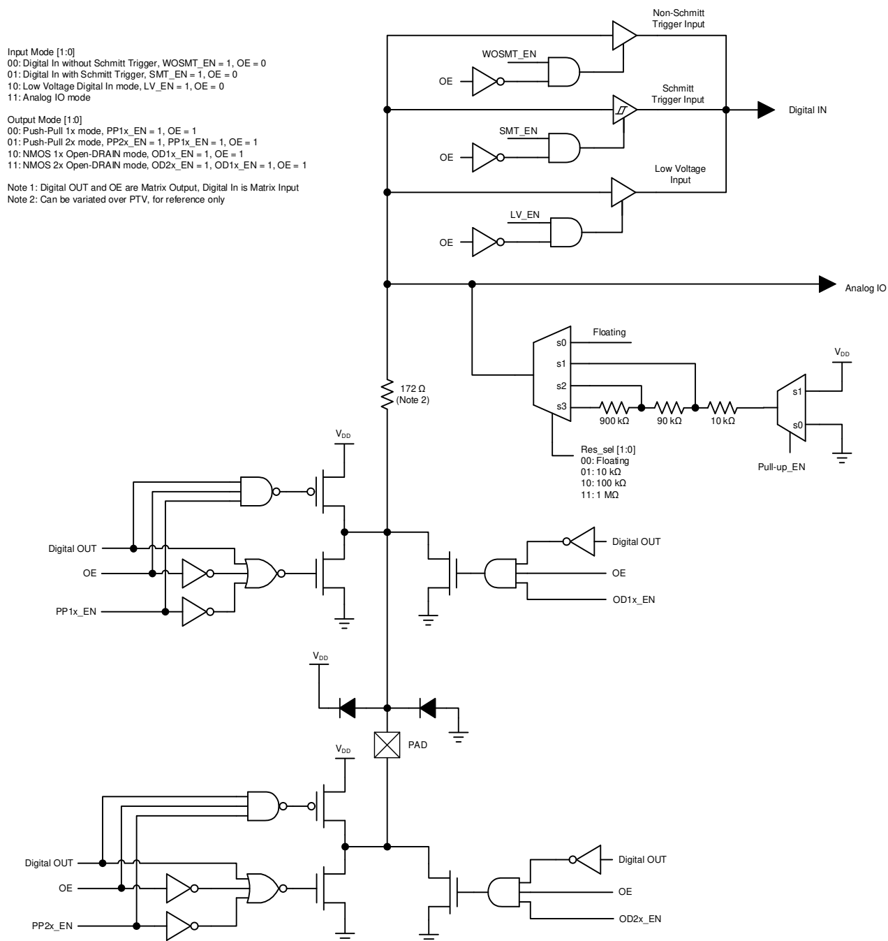
Figure 5: GPIO Matrix OE IO Structure Diagram
