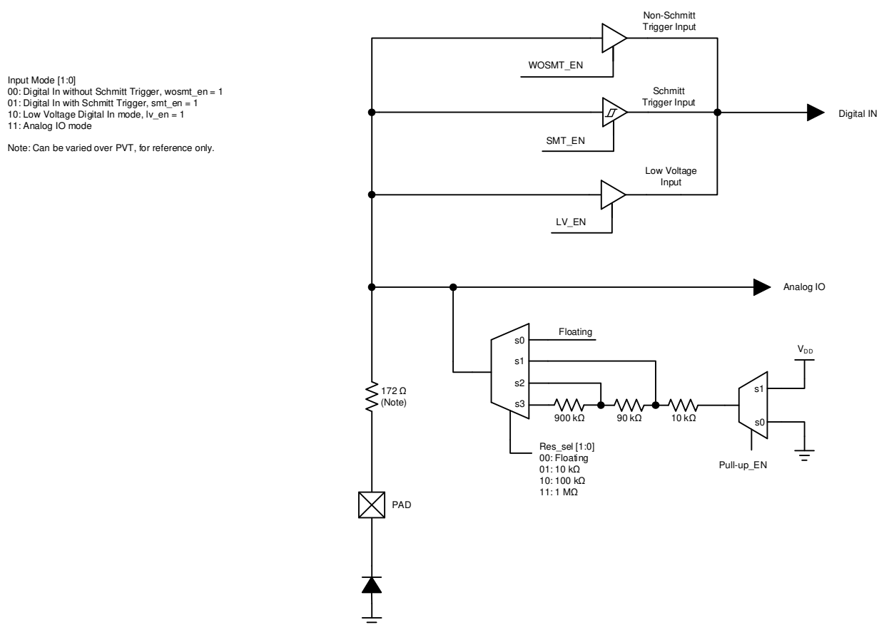
Figure 3: GPI Structure Diagram
