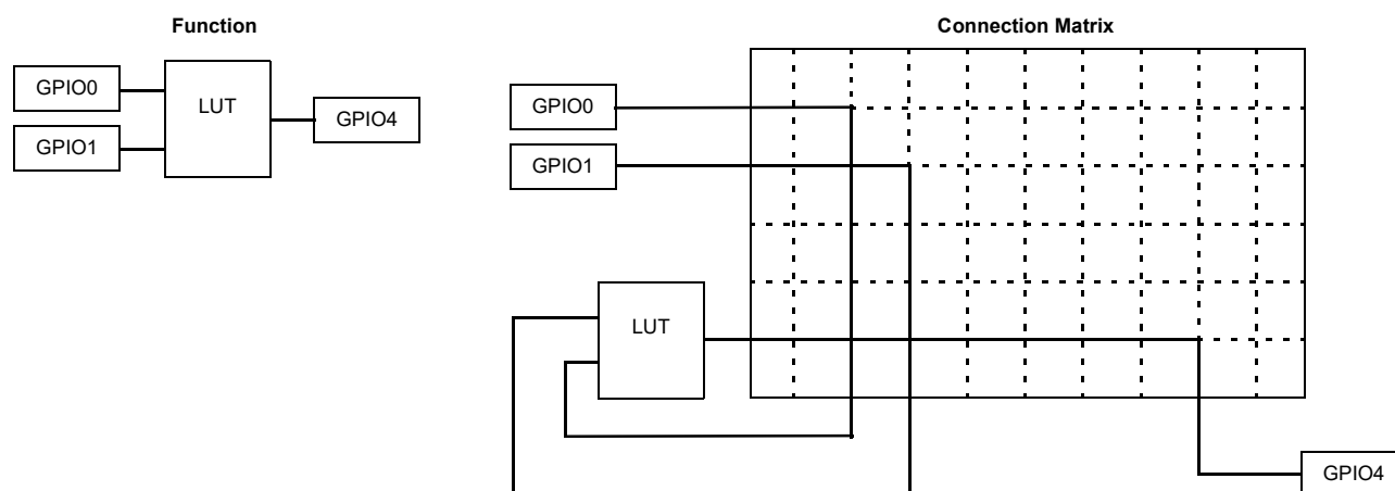
Figure 47: Connection Matrix Example
