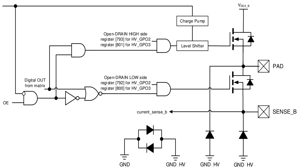
Figure 7: HV GPO Matrix OE IO Structure Diagram (for HV GPOs 2 and 3)
