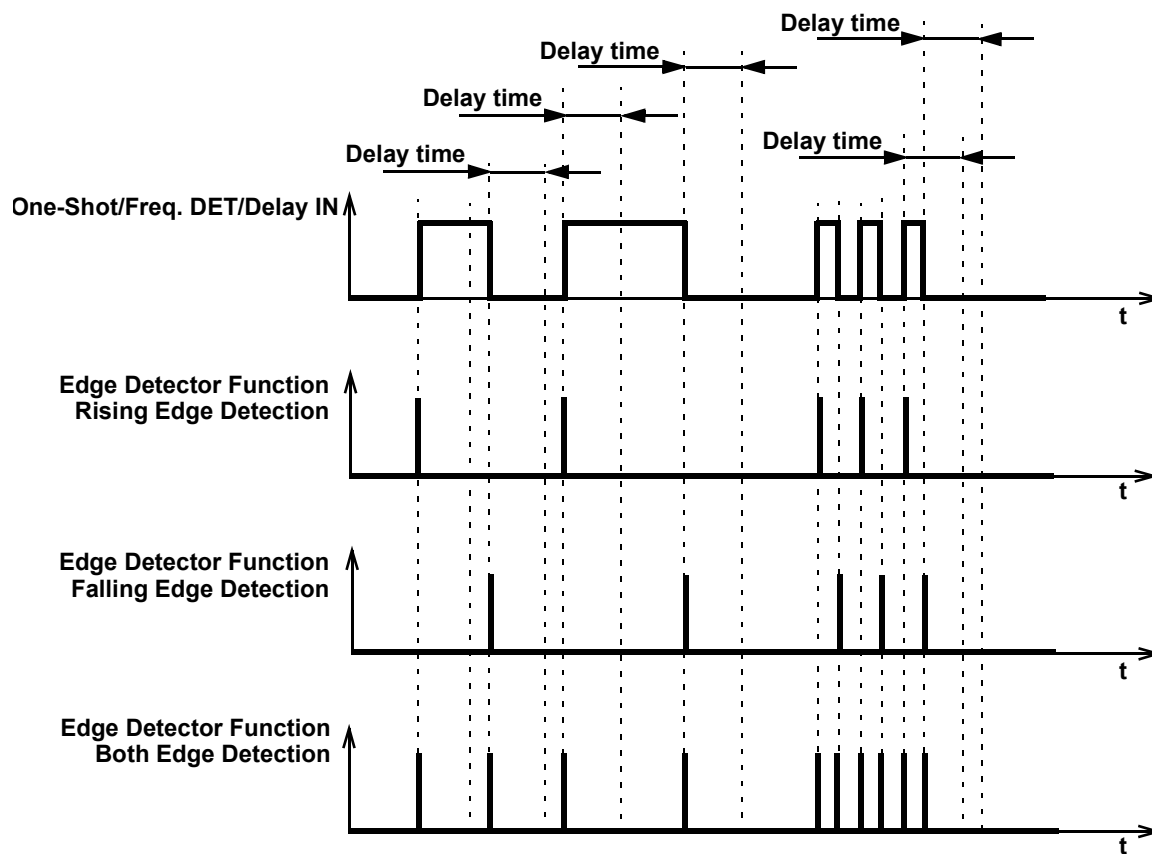
Figure 86: Edge Detection Mode Timing Diagram
