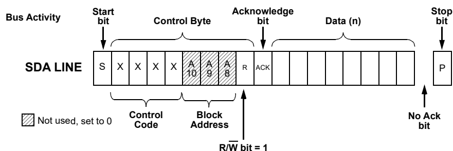
Figure 152: Current Address Read Command, \overline{R/W} = 1
