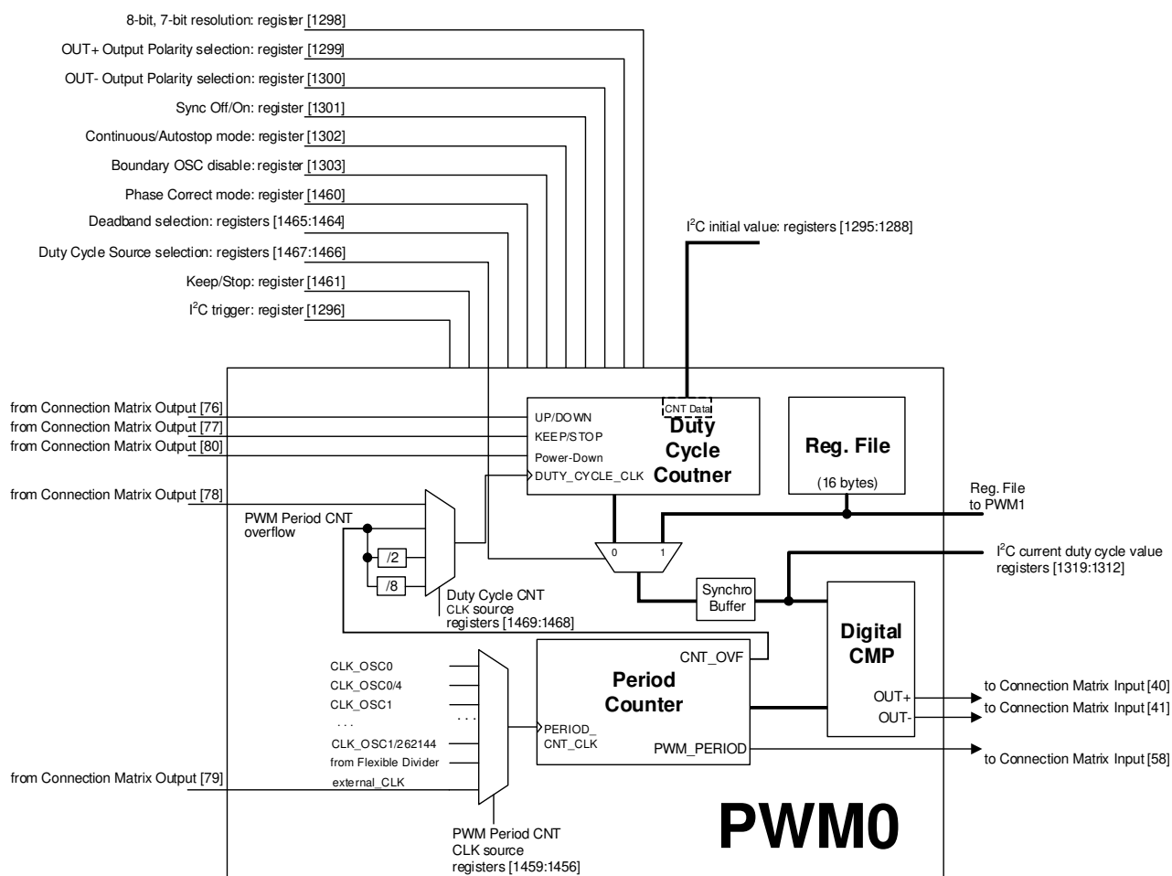
Figure 108: PWM0 Functional Diagram
