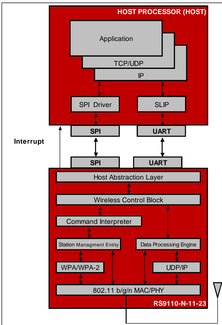
Figure 10: RS9110-N-11-23 Software Architecture Block Diagram
