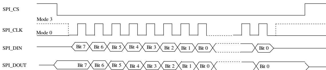
Figure 7: SPI Protocol
