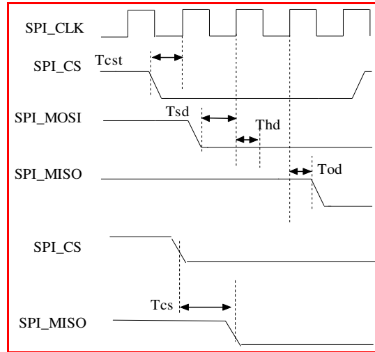
Figure 9: Interface Timings – SPI Interface High-speed Mode
