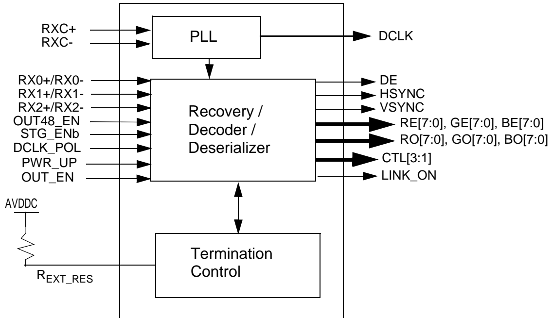
Figure 2-1 Block Diagram of DVI Receiver EP161
